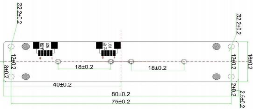
BOTTOM VIEW
