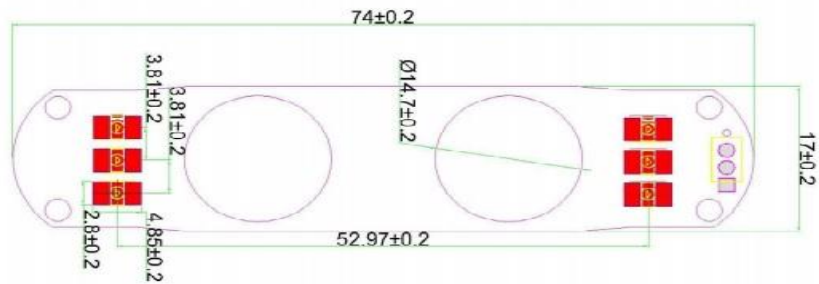
TOP VIEW (LED)
